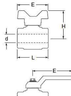
Handle construction for sizes 1¼" - 2"
